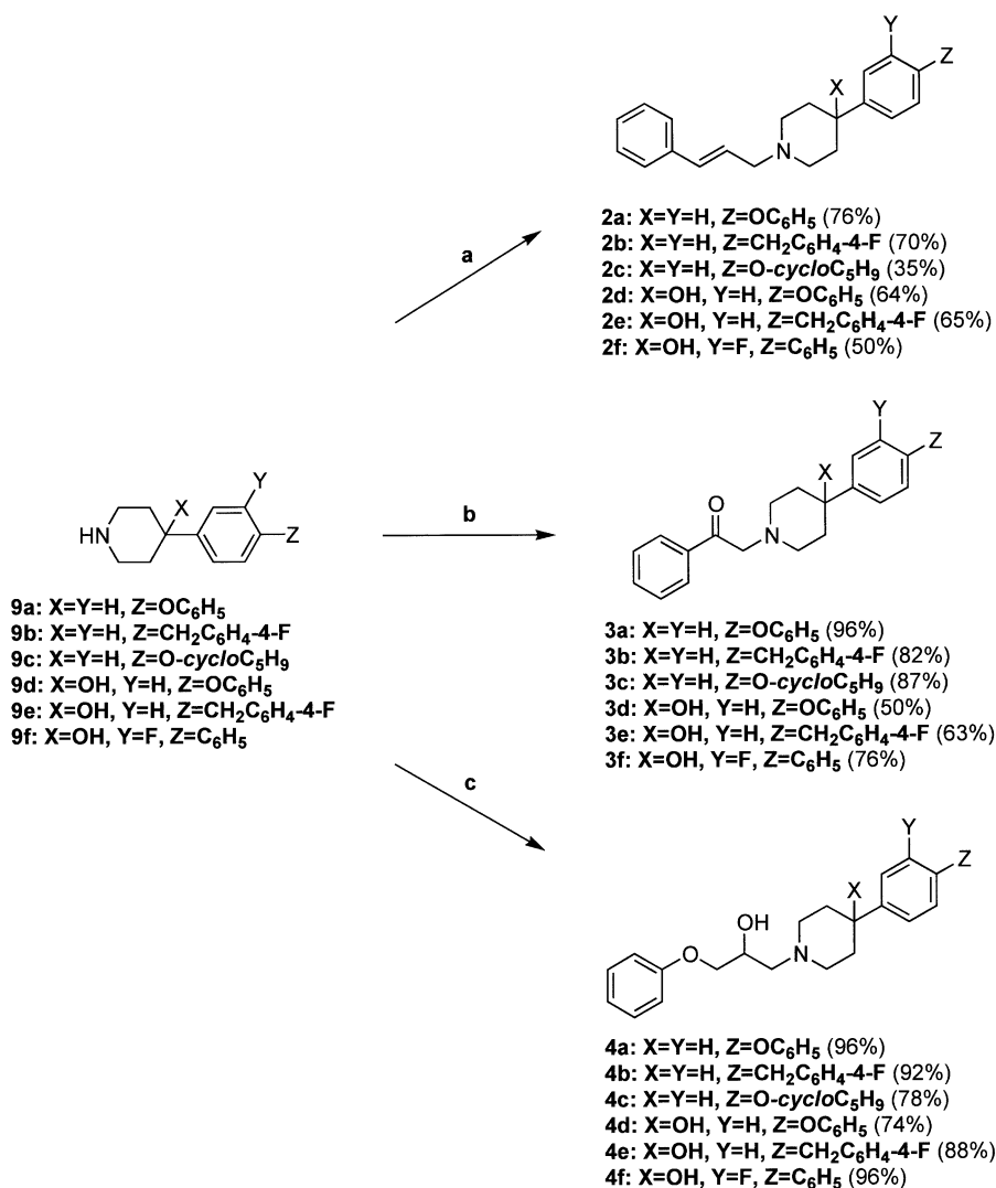
Scheme 2. Reagents and conditions: (a) cinnamyl bromide, Et 3 N, MeCN, 80 °C, 2 h; (b) phenacyl bromide, Et 3 N, MeCN, 80 °C, 2 h; (c) phenyl glycidyl ether, 2-PrOH, reflux, 2 h.
